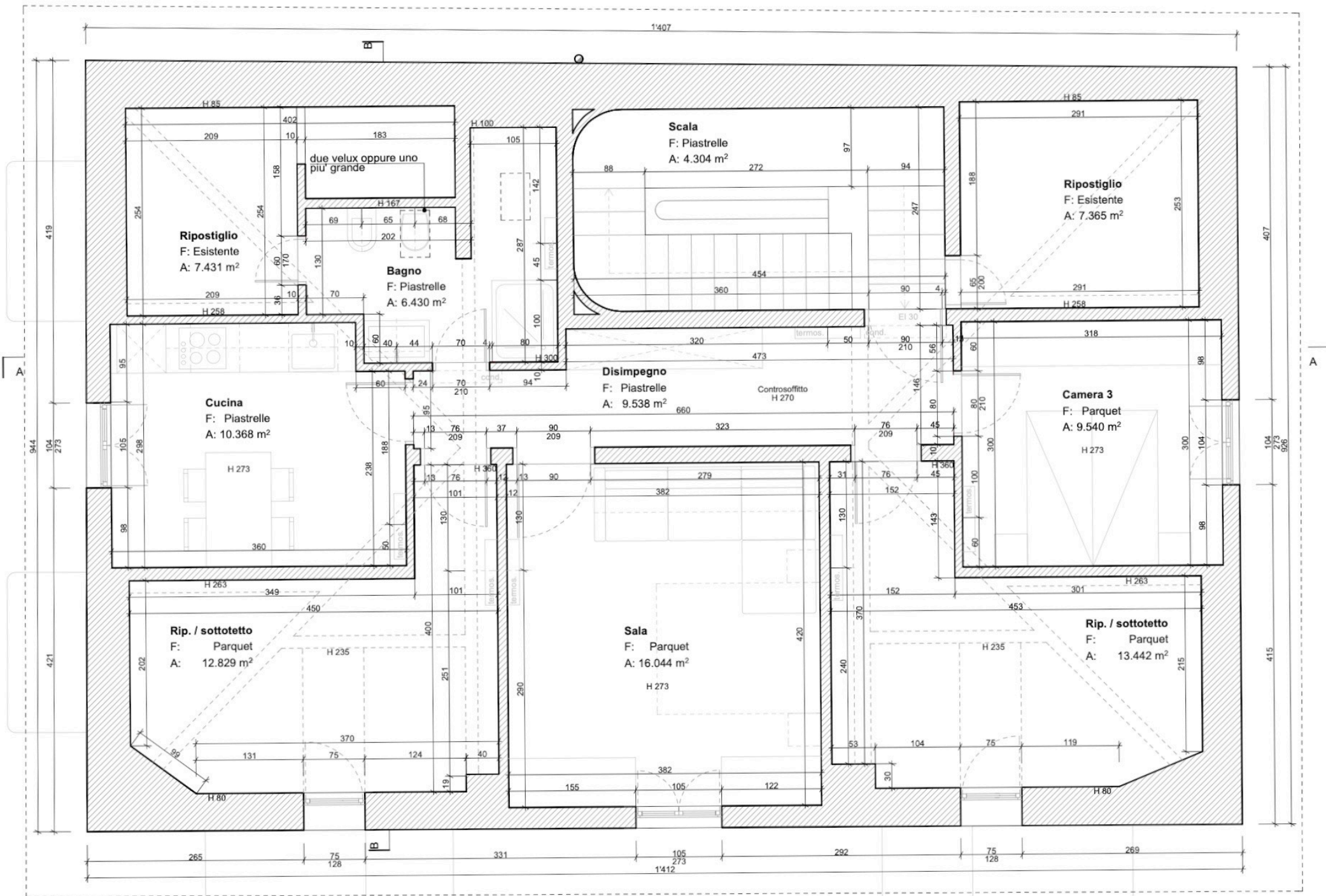
Piano Mansarda - Scala 1:50
